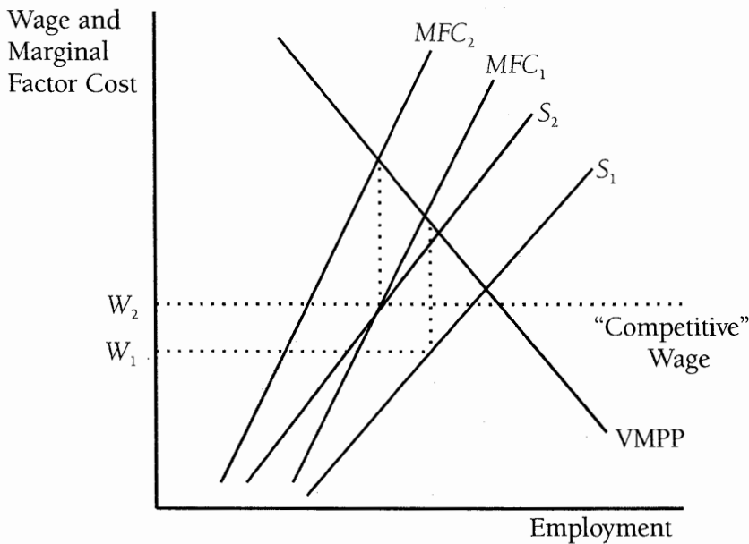
Figure 3 Short Run Effect of Search Costs
